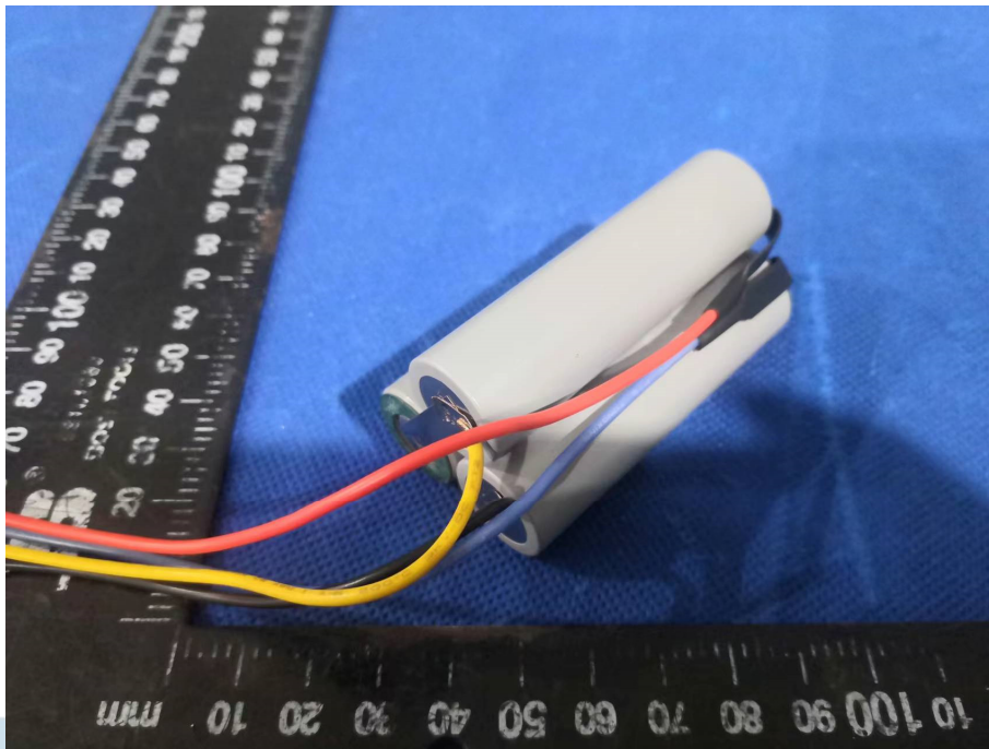
Fig.3 Battery disassembled-1
